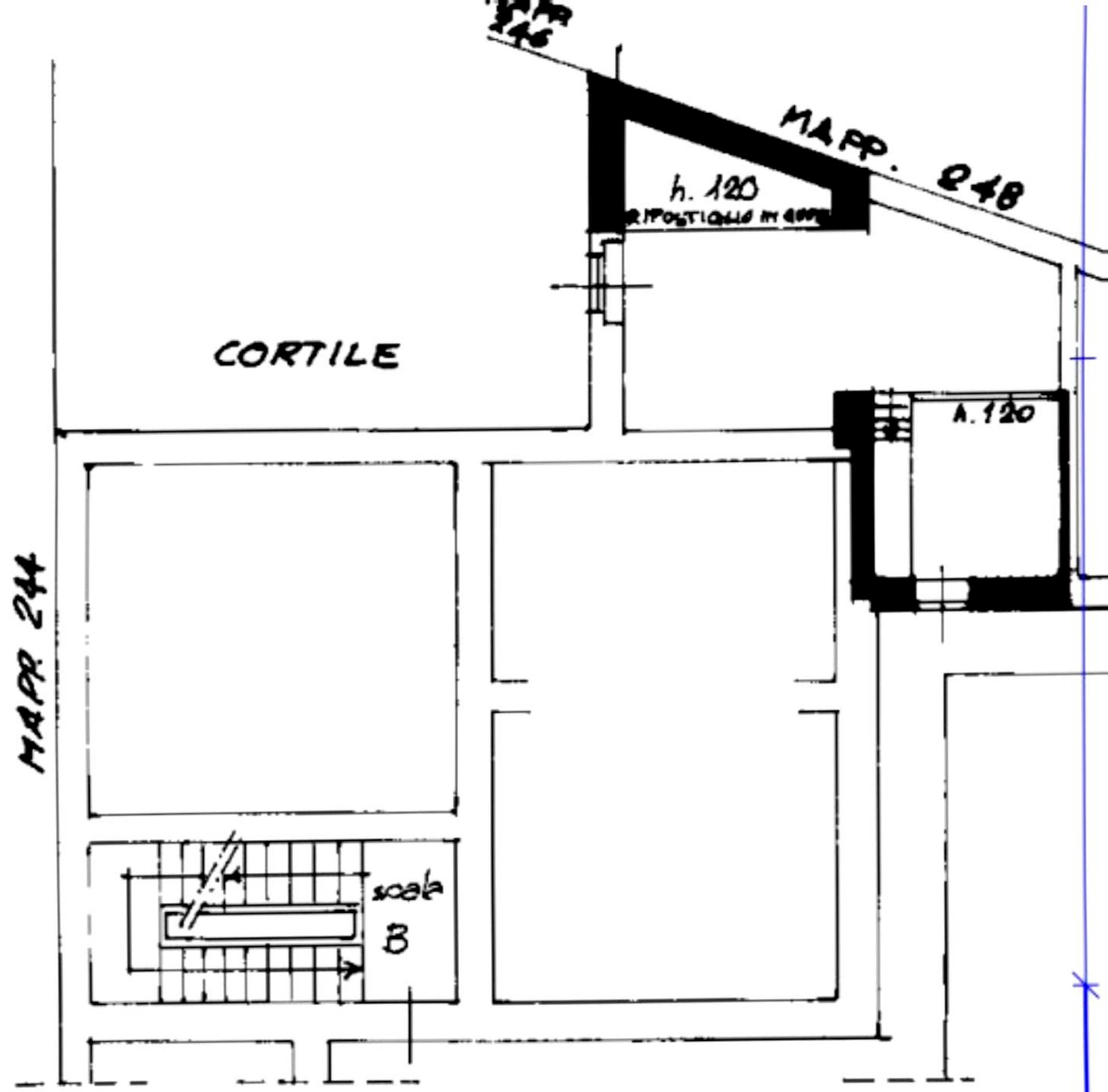
PIANO SOPRALCO
